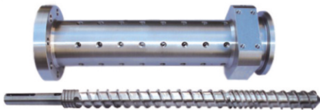
■ Rubber Screw & Barrel
